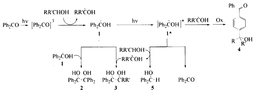
Scheme 1. Reactions of the ground-state and electronically excited hydroxydiphenylmethyl radical (1)
