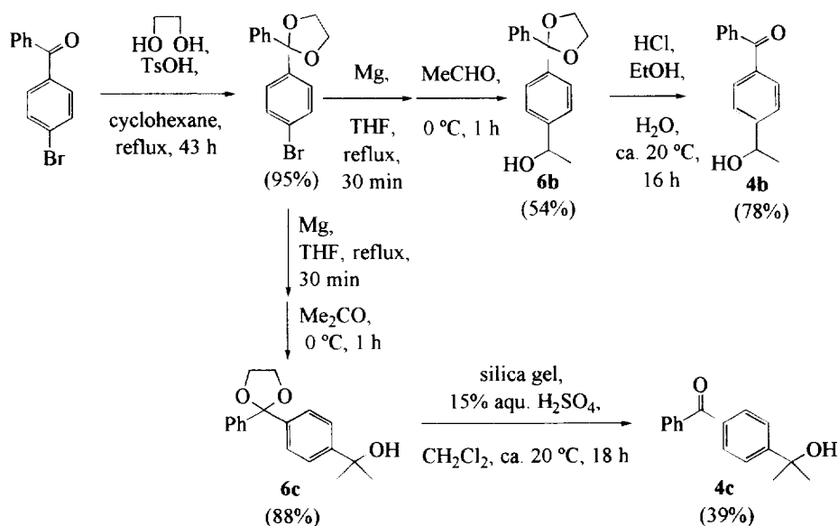
Scheme 2. Synthesis of the cross-coupling products 4b and 4c
